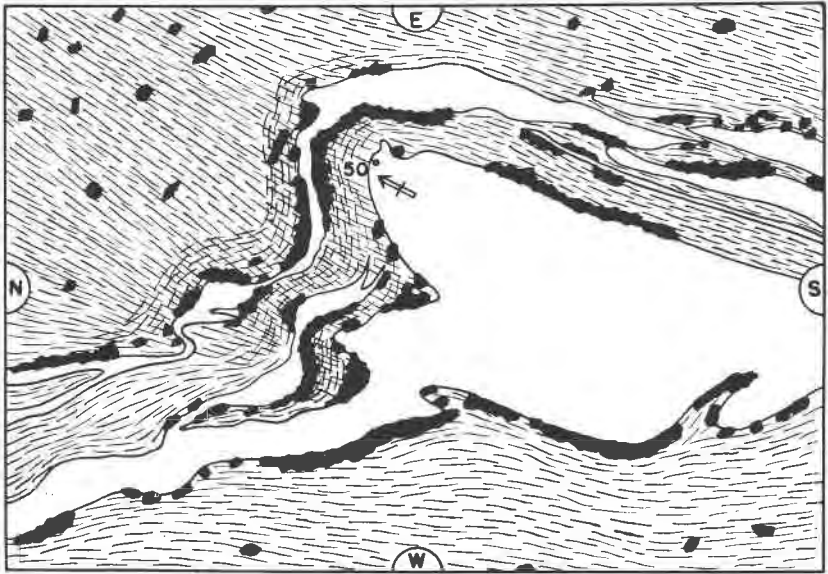
FIG. 2. Map of quartz veins in schist showing staurolite layers. West slope of Croydon Mtn in Croydon, New Hampshire. Area about three feet by four feet. Staurolite—black, quartz veins—clear, schist—lined. Arrow shows attitude and plunge value of folds. Intersecting lines show regional schistosity cutting bedding.
