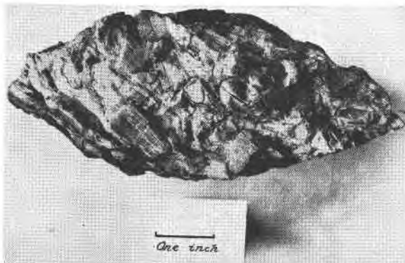
FIG. 1. Kyanite pegmatite from Shepherd mine, Masons Mountain, North Carolina. The warped strip in the right central part of the specimen is biotite. Other blades are kyanite in quartz-kaolinized feldspar matrix.
