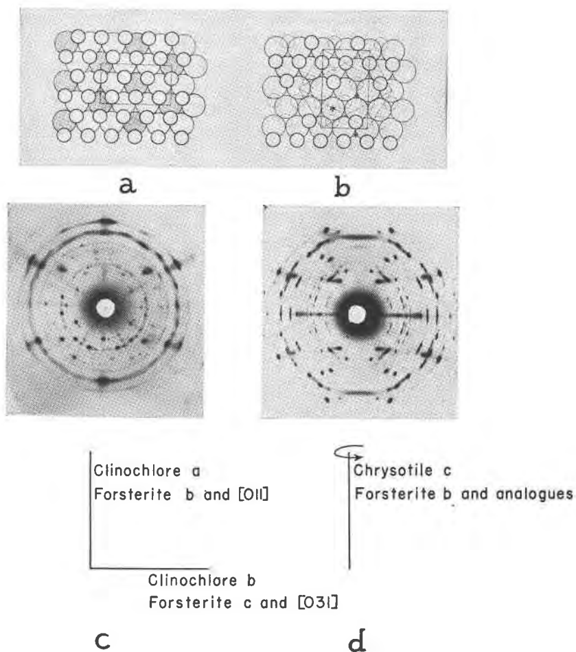
FIG. 2. The relationship of corresponding octahedrally coordinated levels in (a) clinocllore or chrysothile and in (b) forsterite. The diffraction diagram (c) represents a view along c for clinocllore or a for the forsterite growths. The diagram (d) is the synthetic fibrous forsterite product. In each case sufficient diffraction features of the respective unreacted starting materials show in the diagrams to mark the relative orientation before and after firing.
