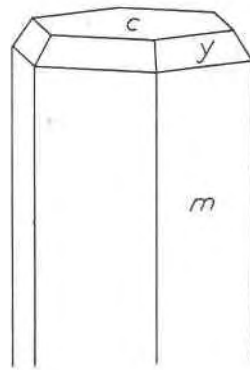
FIG. 2. Pyromorphite.
