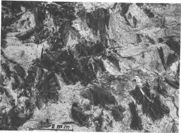
FIG. 1. Chloritoid schist near Rawlinsville, Lancaster County, Pennsylvania. The dark mineral is chloritoid.
