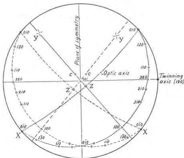
FIG. 3. Optic orientation of the two twinned lamellae in a chloritoid from Lancaster County. The twinning axis is the zone-axis [120]. X = b , c = c axis.
