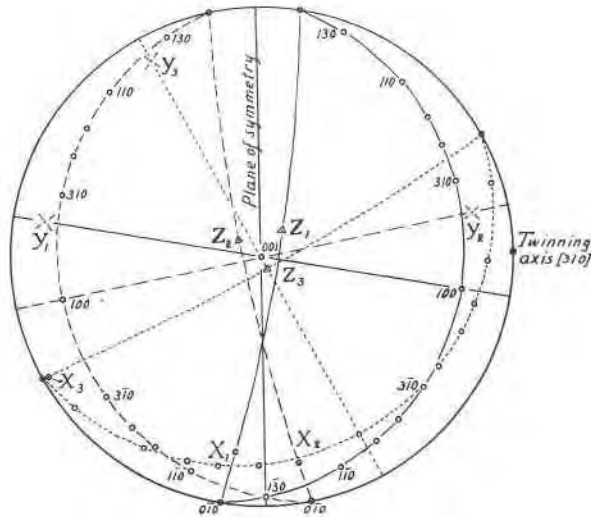
FIG. 5. Orientation of three sets of lamellae in a chloritoid from Lancaster County. Two sets are clearly triclinic and twinned; the third set is very nearly monoclinic.
