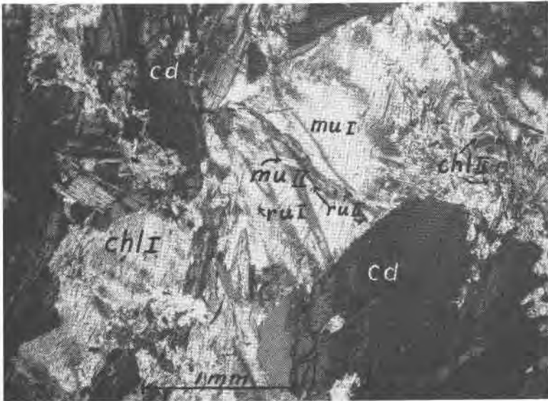
FIG. 2. Twinning in chloritoid (cd) from Lancaster County. Second generation muscovite (mu II), chlorite (chl II), and rutile (ru II) transect the older wrinkled muscovite (mu I) and chlorite (chl I).
