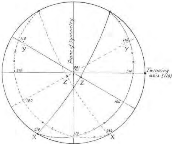
FIG. 4. Orientation of two sets of twinning lamellae in a chloritoid from the same thin section as Fig. 1. Twinning axis is [110] . X = b .
