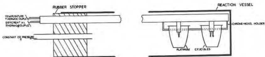
FIG. 1. Reaction vessel with DTA sample holder.
