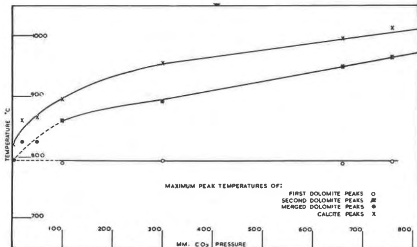
FIG. 4. Maximum differential thermal peak temperatures of dolomite and calcite at various \text{CO}_2 pressures.
