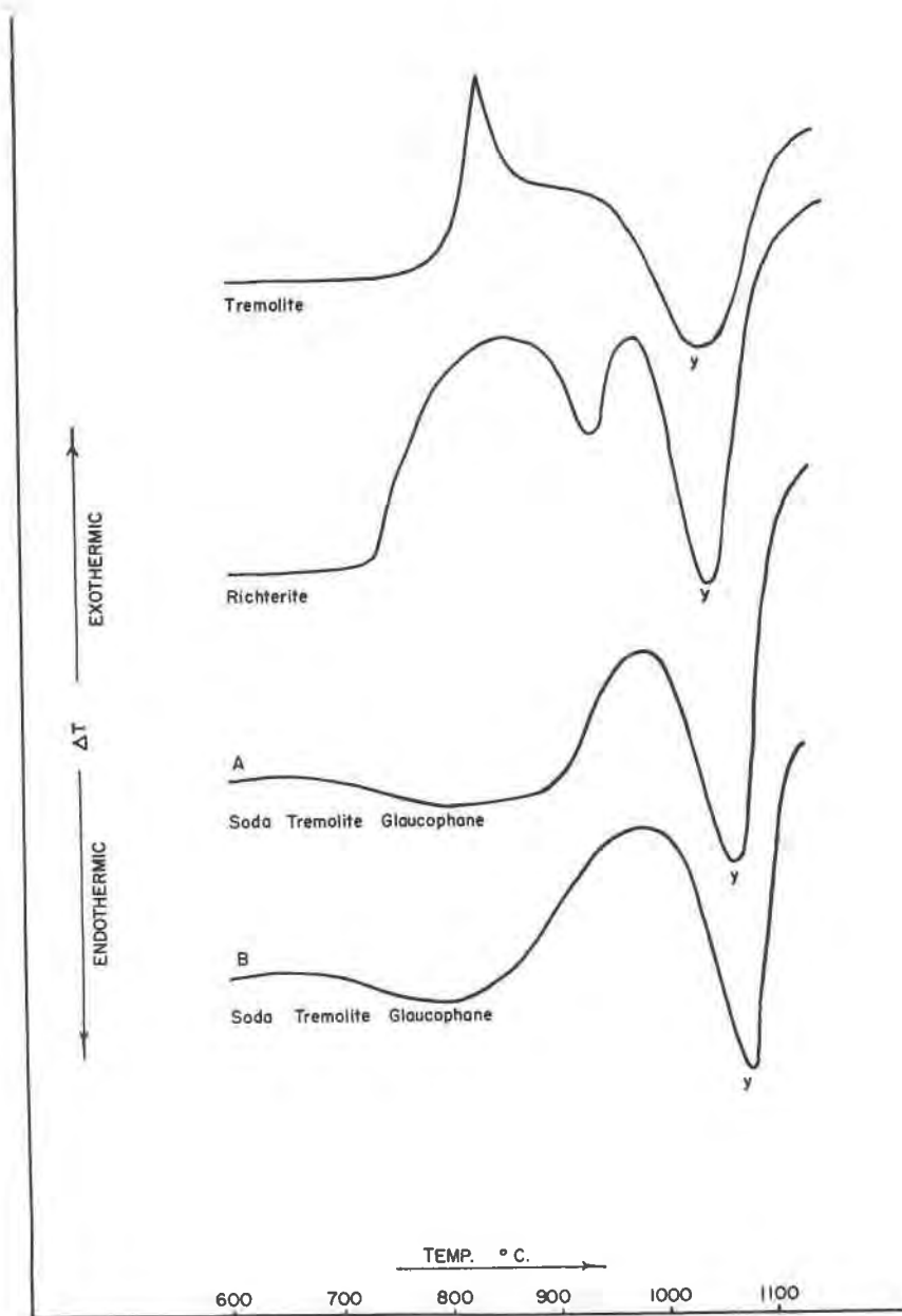
FIG. 1. Thermographic curves of amphiboles.
