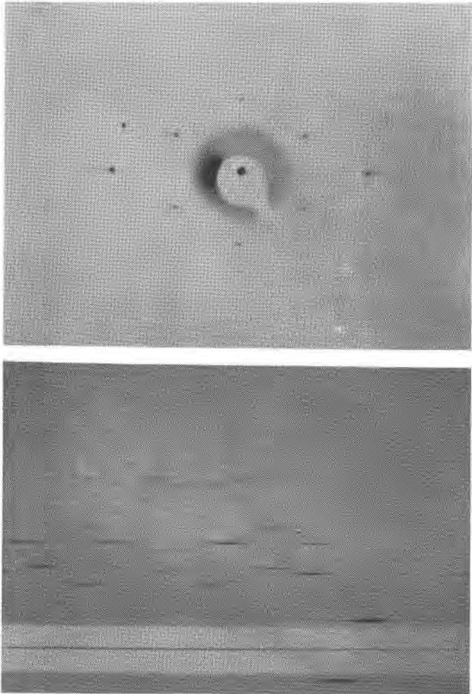
FIG. 1 (top). Metaheewettite. Precession photograph of zero level (approximately normal to (101) axis) showing double set of reciprocal lattice points, (hk)^* , (\bar{h}l)^* .* (Mo, 36 hrs.)
