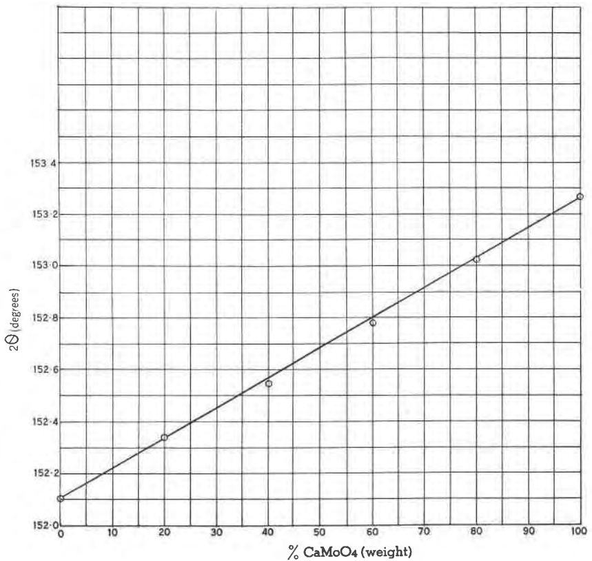
FIG. 4. Variation of 2\theta for line No. 1 with variation in the chemical composition of the scheelite-powellite series.
