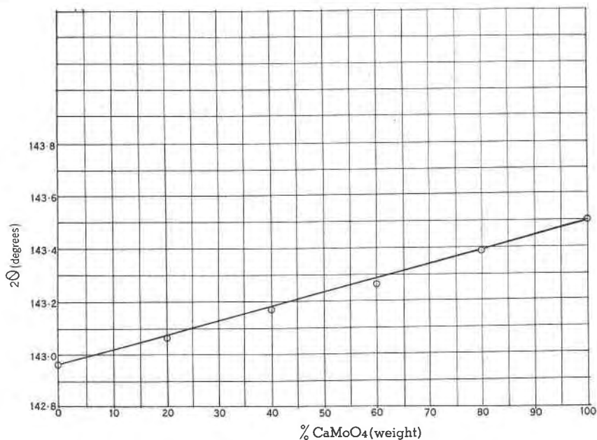
FIG. 6. Variation of 2\theta for line No. 3 with the chemical composition in the scheelite-powellite series.
