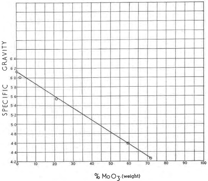
FIG. 1. Graphical representation of the variation of the specific gravity of members of the \text{CaWO}_4\text{-CaMoO}_4 series. No specific gravity determinations was attempted on the synthesized members because of their very fine grain size.
