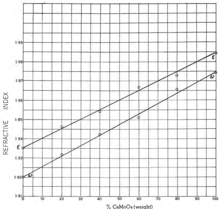
FIG. 2. Graphical representation of the variations of the refractive indices \omega and \epsilon with the chemical composition of the synthetic \text{CaWO}_4 - \text{CaMoO}_4 series.
