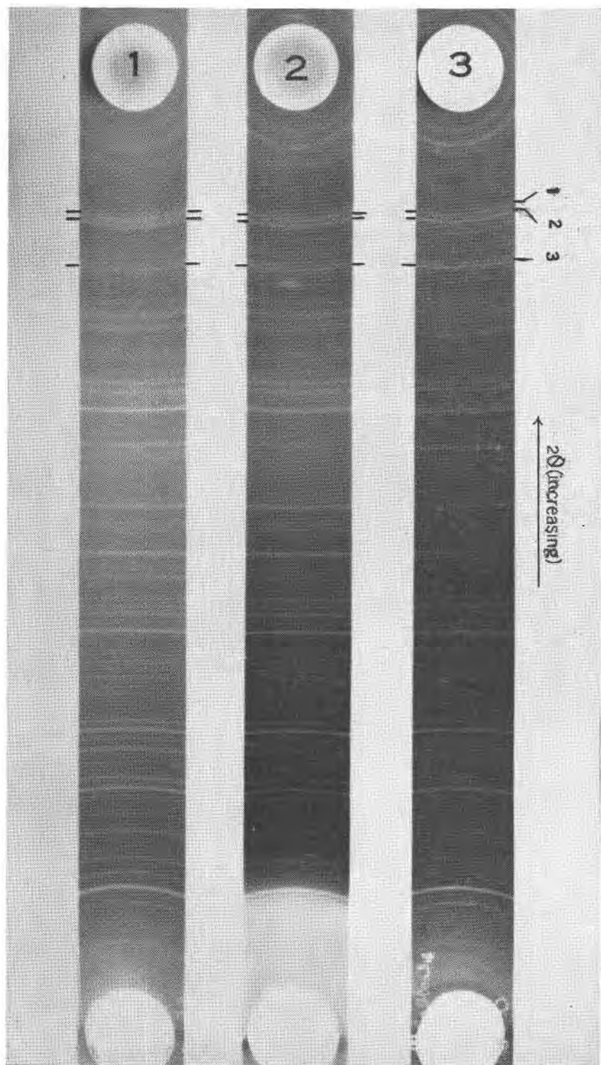
Fig. 3. X-Ray powder patterns of: 1. Natural scheelite, 2. Synthetic \text{CaWO}_4 , 3. Synthetic \text{CaMoO}_4 .
