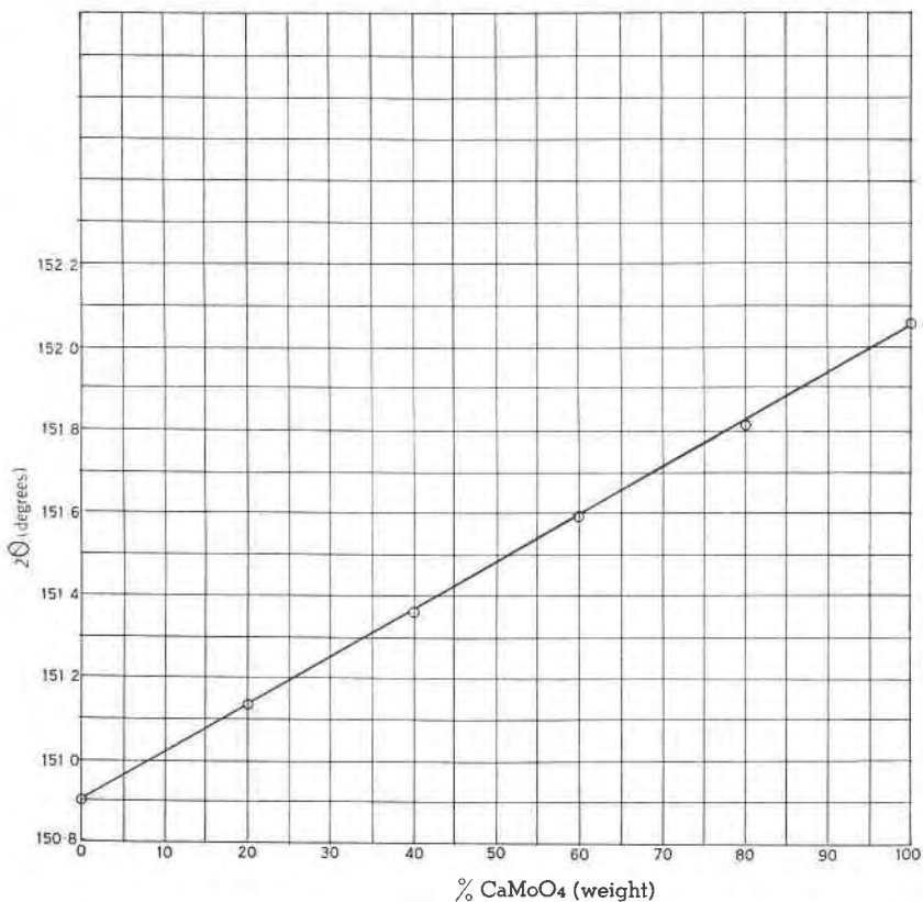
FIG. 5. Variation of 2\theta for line No. 2 with variation in the chemical composition of the scheelite-powellite series.
