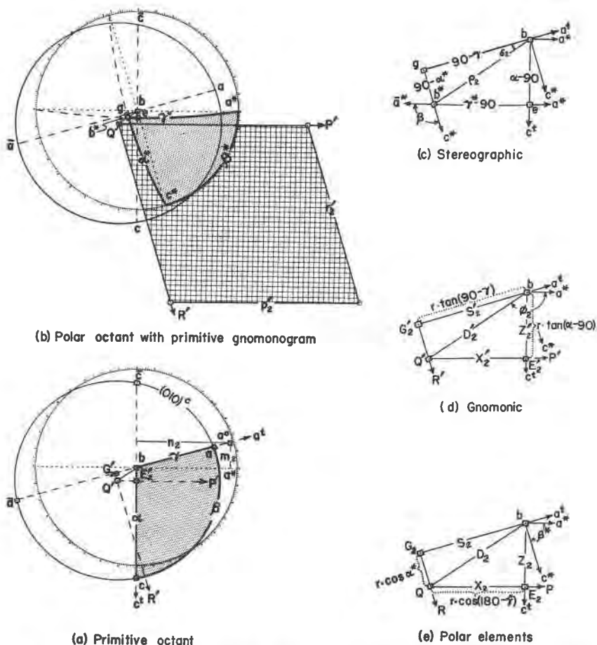
FIG. 3. Gnomonostereogram of chalcantite, second permutation. a. The entire projection with primitive circle (graduated) of r=1 . The primitive octant is stippled. b. The entire projection with primitive of r=1 . The polar octant is stippled and the primitive gnomonogram is reticulated. c. Central portion of stereoprojection (see b ) with r=10 . d. Central portion of gnomonogram with r=5 . Note that distances D_2' , S_2' , X_2' , and Z_2' are capitalized to emphasize that r \neq 1 . e. Central portion of polar elements plane with r=5 . Here also D_2 , S_2 , X_2 , and Z_2 are capitalized, since r \neq 1 .
