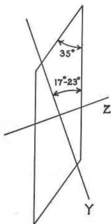
FIG. 1. Optical Orientation of Uranopilite.
