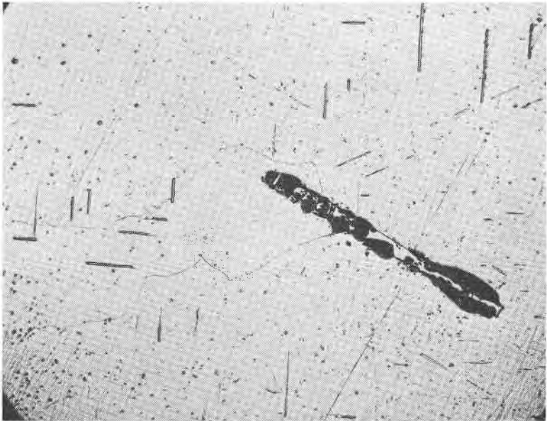
FIG. 7. The big inclusion is rhabdite, perhaps large enough to be called schreibersite, the dark spots are due to chipping in the preparation of the surface. If the plane of the picture is parallel to 001, the small rhabdites at right angles to each other lie along the cube face and the large phosphide body and the other rhabdites are parallel to trapezohedral faces. \times 40 .
