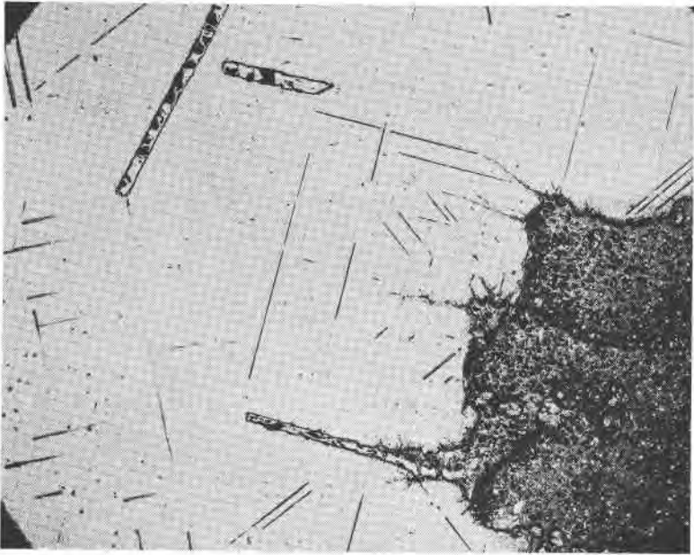
FIG. 9. The troilite at lower right is darkened by carbon, lacks a sharp border, and occasionally phosphide rods extend as prongs from the edges of the FeS. Four sets of Neumann lines are shown in the kamacite. \times 40 .
