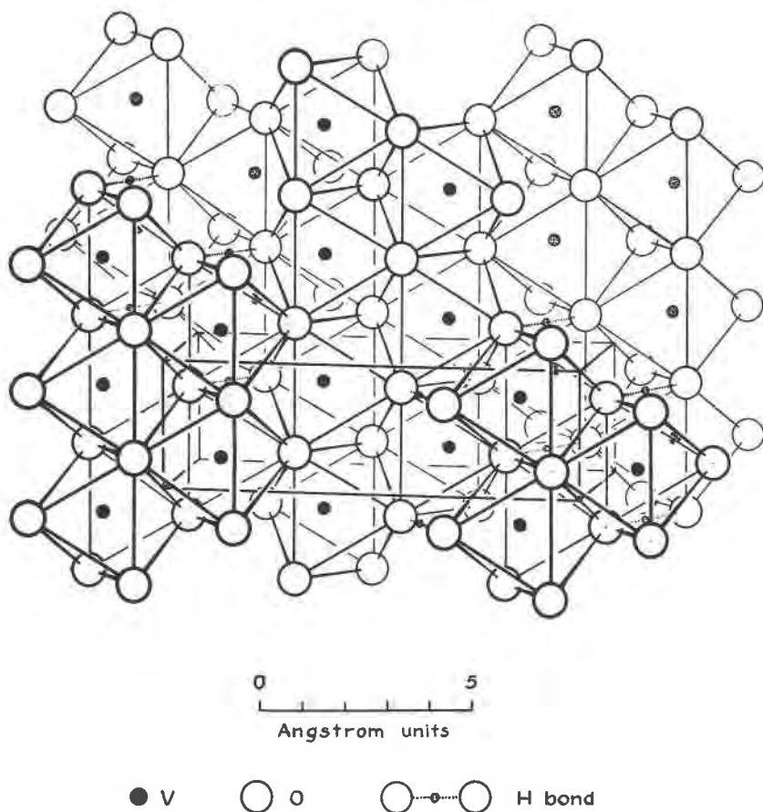
FIG. 2. Pictorial view of crystal structure of montroseite.
