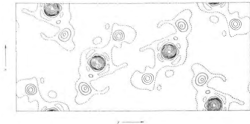
FIG. 1. Electron density projection along [001] of montroseite.
