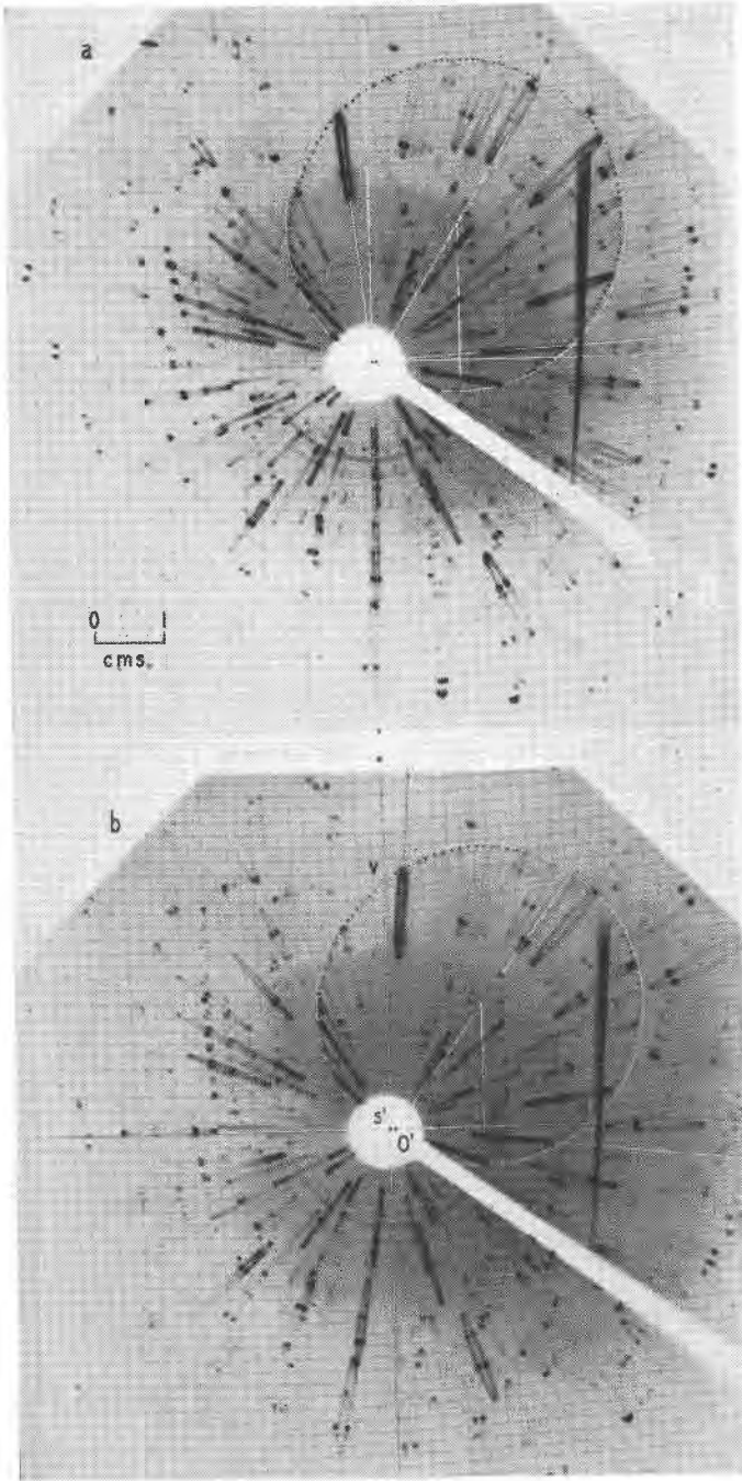
FIG. 40. Precession orientation photos of hopeite with \mu = 3^\circ and Mo radiation at F = 60.00 mm. If correctly oriented, precession would be on [a], with [c] parallel to the dial axis. Here the dial reading is off 15^\circ (up), the H-arc off 10^\circ (to the right), and the V-arc off 5^\circ ; this last error is up in (a) and down in (b).
