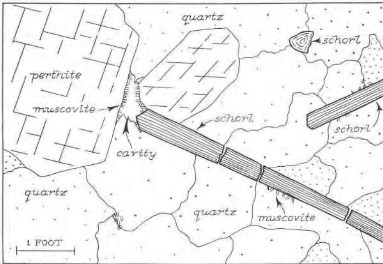
FIG. 9. Giant pegmatitic texture in quartz—perthite—schorl core of large pegmatite dike near Sage, Riverside County, California. The large crystals show smooth faces where they form the walls of the small cavity. Contacts between anhedral quartz crystals are diagrammatic, but positions of most are correct to within an inch.
