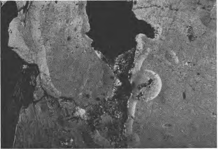
FIG. 7. Highly inclined, plane-polarized light; mag. 66X. This section contains quartz, biotite, plagioclase and finer-grained alteration product. Note in particular the wets in the quartz and the elliptically-shaped low-relief area. These are apparently related to alteration zones in the quartz which now are filled with a fine-grained muscovite-like product. These circular "depressions" are thought to be cross sections of the sinuous channels seen in this and other thin sections. The channel in the oligoclase appears to be independent of any crystallographic direction.
