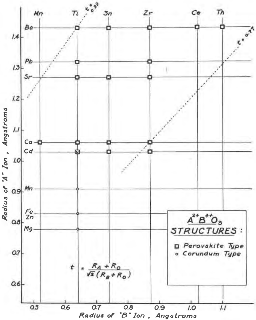
FIG. 2. Distribution of A^{2+}B^{4+}O_3 Structures in Relation to Cation Radii.
