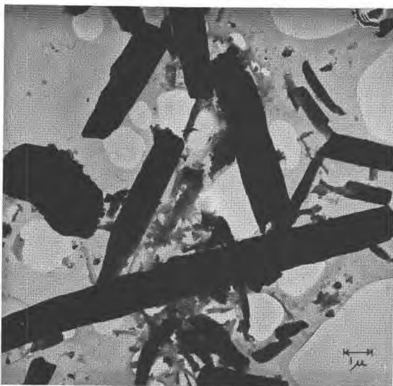
FIG. 2. Electron micrograph of crystallites showing their acicular nature and characteristic cleavage at the end of needles. Mag. 7,500 \times
