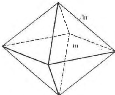
FIG. 4. Callaghanite, clinographic projection showing the forms \{111\} and \{\bar{1}\bar{1}1\} .
