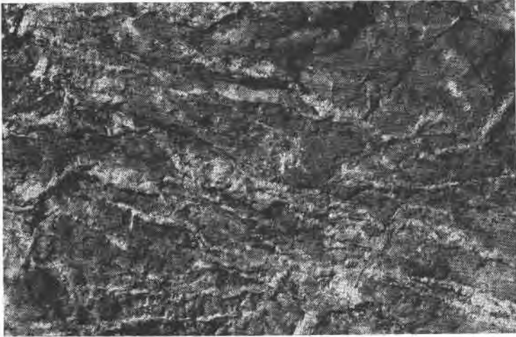
FIG. 1. Weathered surface of pollucite exposed on the surface of a boulder. Note the irregular veins of spodumene with some mica which stand out sharply in relief.
