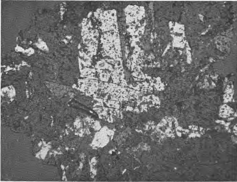
A thin section of Pikes Peak material, in liquid with n=1.347 . Weberite crystals corroded by "cubic" minerals. Mag. 134 \times . Upper nicol a few degrees from crossed position in order to show the surrounding material.
