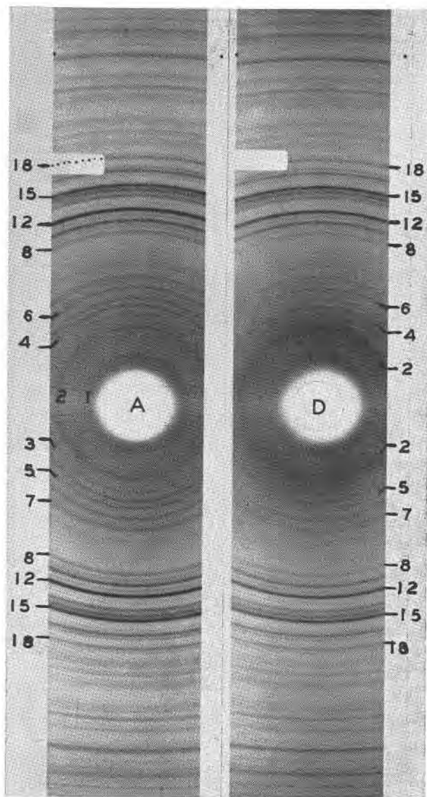
FIG. 1. X-ray powder photos, Fe radiation (Mn filter), 114.6 mm. diam. camera, natural scale. Some of the lines are numbered as in Table 3.
