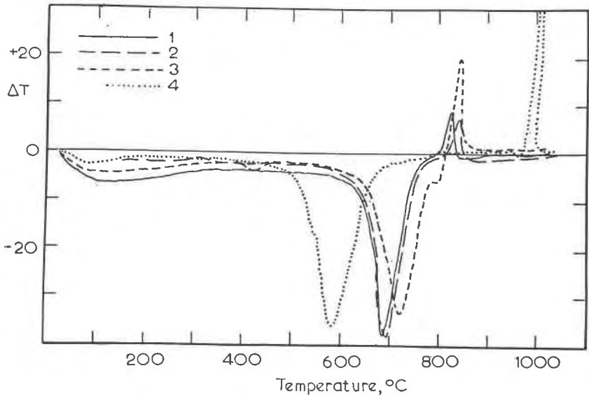
FIG. 6. Differential thermal analysis curves for ortho-antigorites and kaolinite.
