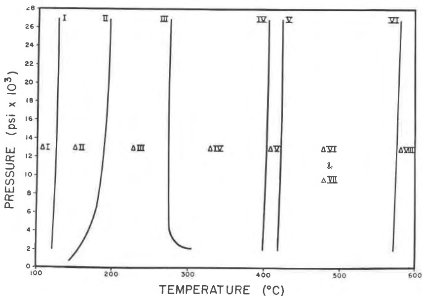
FIG. 7. Univariant curves for the system \text{Al}_2\text{O}_3\text{-SiO}_2\text{-H}_2\text{O} . The triangle numbers in areas between curves refer to triangles in Fig. 6. Reactions taking place along the curves are as follows: I, \text{Gibbsite} \rightleftharpoons \text{boehmite} + \text{H}_2\text{O} ; II, \text{Endellite} \rightarrow \text{halloysite} + \text{H}_2\text{O} ; III, \text{boehmite} \rightleftharpoons \text{diaspore} ; IV, \text{diaspore} \rightleftharpoons \text{corundum} + \text{H}_2\text{O} , and \text{kaolinite} \rightleftharpoons \text{hydralsite} + \text{pyrophyllite} + \text{montmorillonite} ; V, \text{montmorillonite} \rightleftharpoons \text{pyrophyllite} + \text{hydralsite} + \text{H}_2\text{O} ; VI, \text{pyrophyllite} \rightleftharpoons \text{mullite (or andalusite)} + \text{quartz} + \text{H}_2\text{O} .
