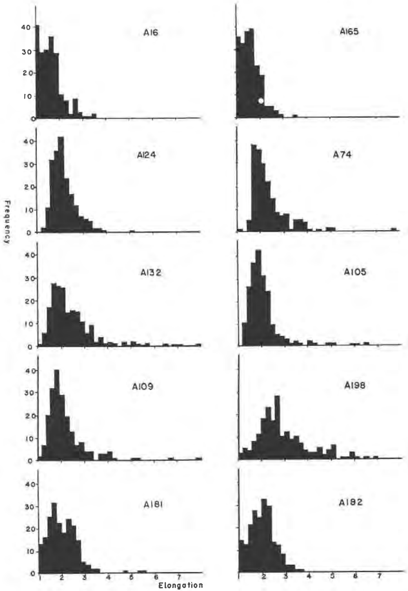
FIG. 1. Frequency-elongation histograms of zircons.
