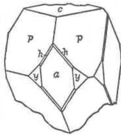
Fig. 5. Apophyllite
