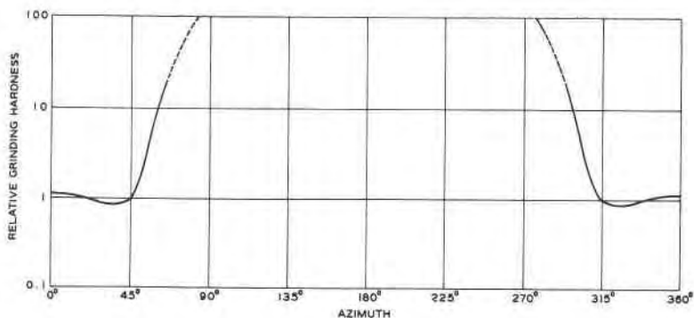
FIG. 3. Zone [\bar{1}01] 5^\circ from dodecahedron.
