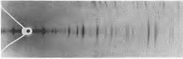
FIG. 2. The zero layer line of a sepiolite fiber x-ray diffraction diagram. Filtered Cu radiation. Camera radius=6.35 cm.
