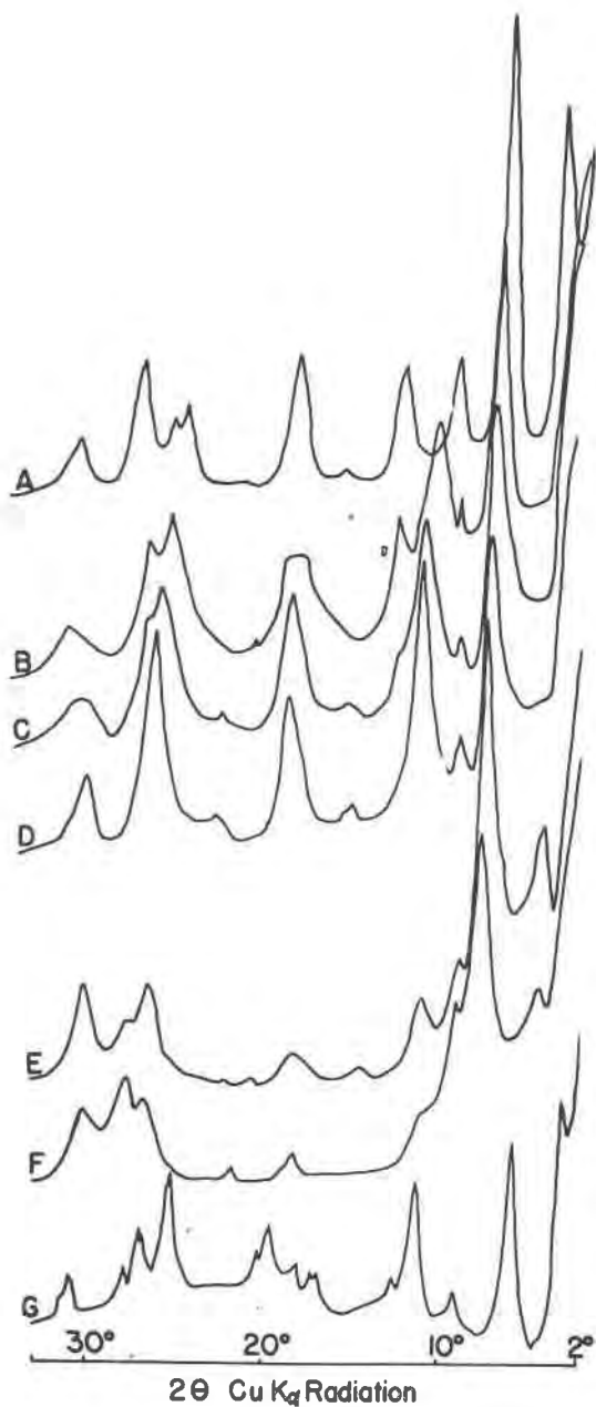
FIG. 1: X-Ray diffractometer patterns of montmorillonite-chlorite from argillaceous siltstone, Ward County, Texas, prepared from < .5\mu fraction by sedimentation on glass slides to yield maximum preferred orientation. A —Unheated, room air; B —85° C., dry air; C —200° C., dry air; D —400° C., room air; E —550° C., room air; F —700° C., room air; G —glycerol saturated, room air.
