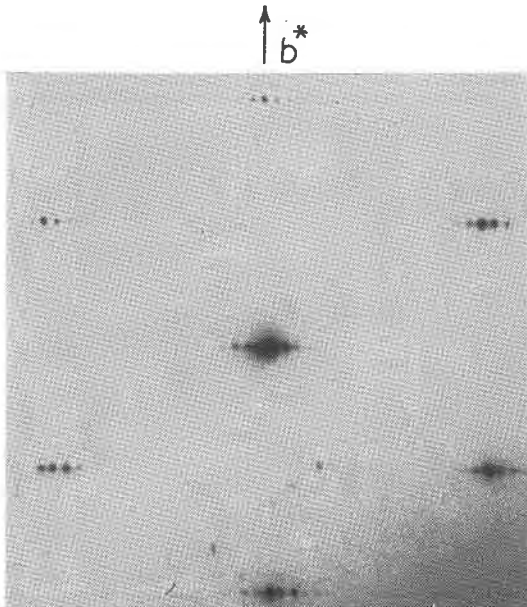
FIG. 5. Antigorite (massive). Part of e.d. pattern from single crystal of Yu Yen Stone, showing very closely spaced spots along a^* corresponding to a \simeq 90 Å. Scale 3\times that of other diffraction patterns.
