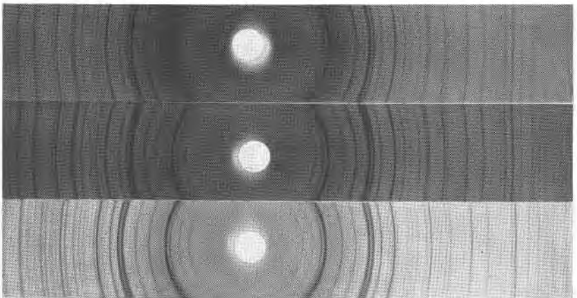
Plate 1. Powder diffraction patterns of cyrilovite, avelinoite, and wardite. (1) Cyrilovite, Cyrilov, Velké Meziříčí, West Moravia; U. S. National Museum 107,425; iron radiation, manganese filter. (2) Avelinoite, Sapucaia pegmatite, Brazil; iron radiation, manganese filter. (3) Wardite, Beryl Mountain, New Hampshire; iron radiation, manganese filter; center of film offset in relation to avelinoite to emphasize difference in cell size.
