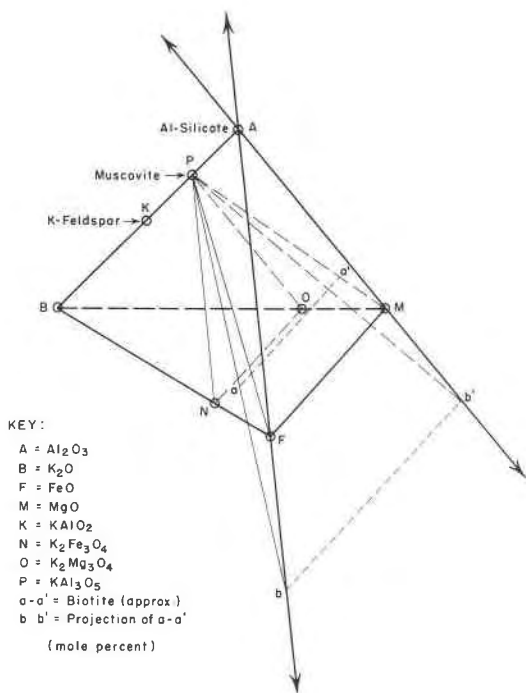
FIG. 3. The tetrahedron Al_2O_3 - K_2O - FeO - MgO showing projection through idealized muscovite composition onto plane determined by Al_2O_3 , FeO and MgO .
