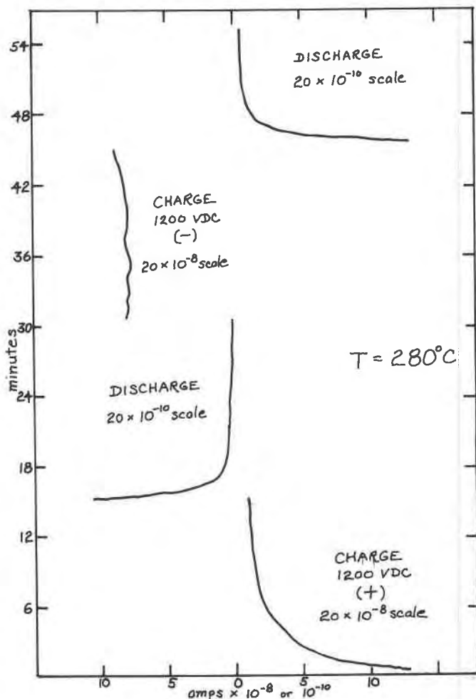
FIG. 8. Current-time curves showing charging and discharging current at 280° C. Note that the scale for the charging current is not the same as that for the discharging current. Traced directly from the Speedomax strip chart.
