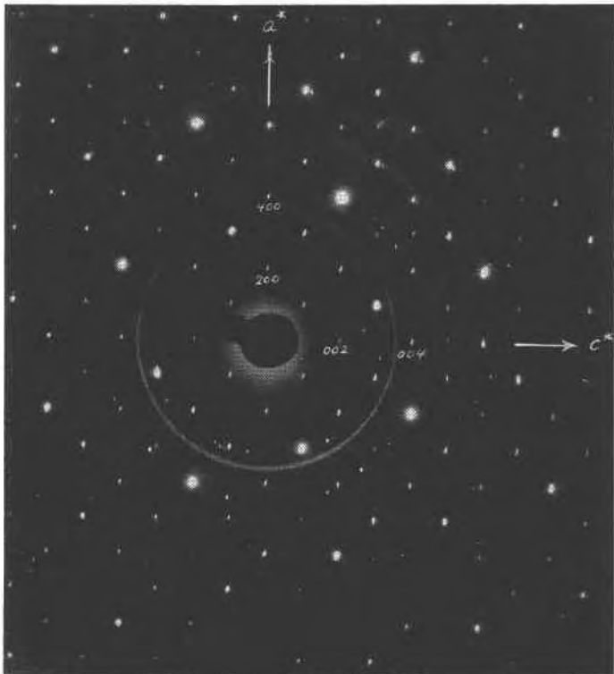
FIG. 2. Electron diffraction spot pattern of simplotite representing the a^*-c^* reciprocal net plane superimposed on an aluminum ring pattern.
