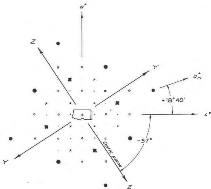
FIG. 3. Schematic drawing showing relation between the reciprocal lattice, optical orientation, and habit of simplotite. Circles represent reciprocal lattice points with k=0 , crosses those with k=1 . (See Fig. 2.) Sketch shows approximate appearance of the crystal on which correlative measurements were made (longest dimension 1 mm.).
