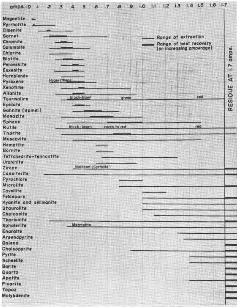
FIG. 1. Magnetic susceptibilities of minerals in Frantz isodynamic magnetic separator (side tilt 15°; forward tilt 25°; dried grains in 100-150 mesh range).
