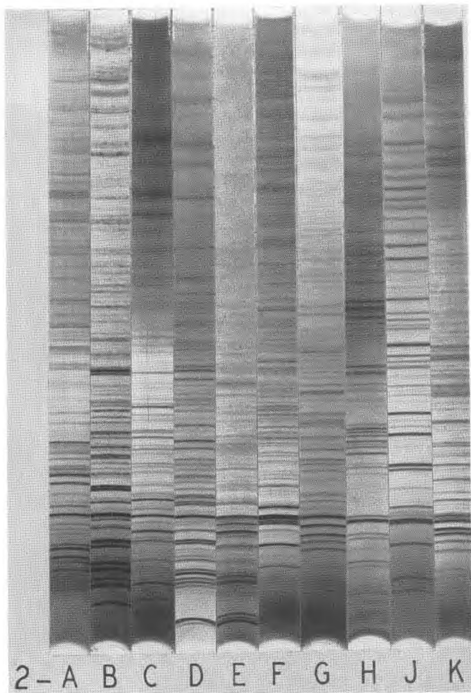
FIG. 2. X-ray diffraction patterns for phosphates whose strongest line corresponds to d of 2.81 to 2.92 Å.
