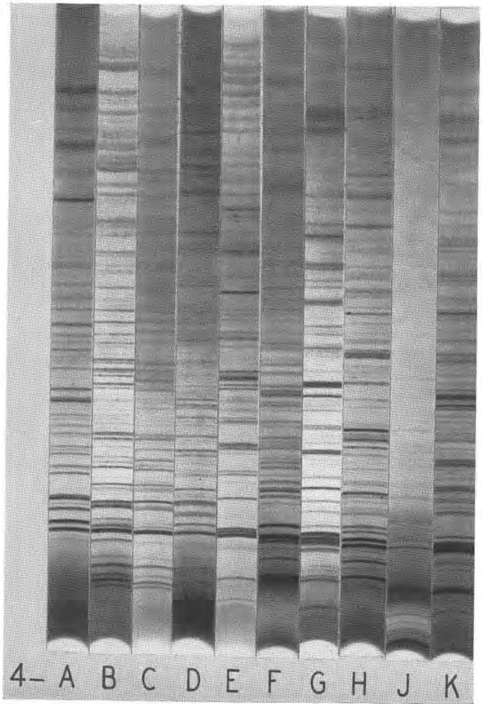
FIG. 4. X-ray diffraction patterns for phosphates whose strongest line corresponds to d of 3.18 to 3.40 Å.
