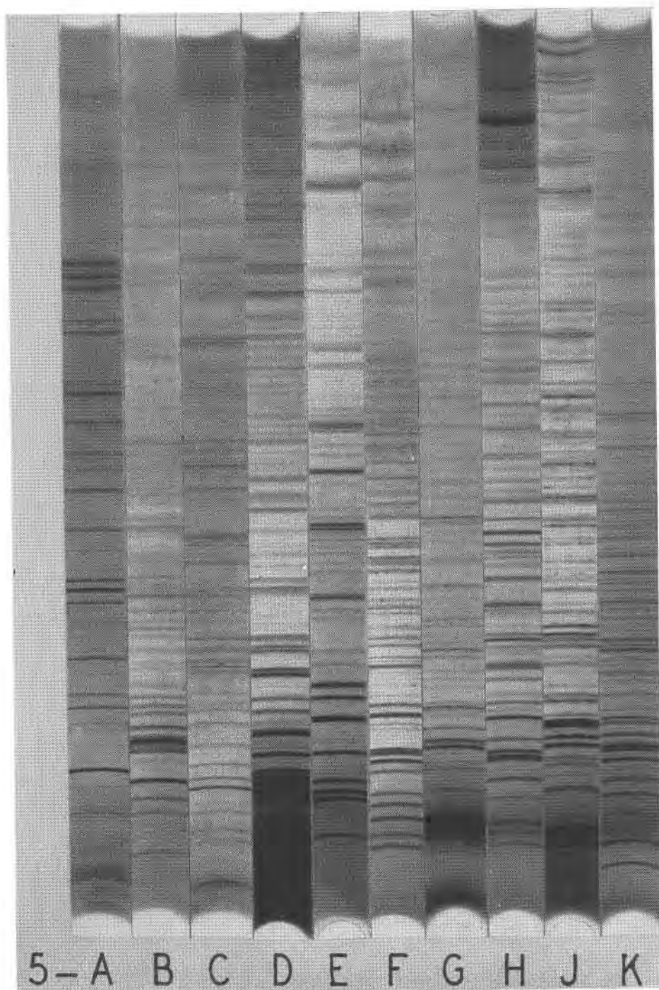
FIG. 5. X-ray diffraction patterns for phosphates whose strongest line corresponds to d of 3.4 to 6.0 Å.
