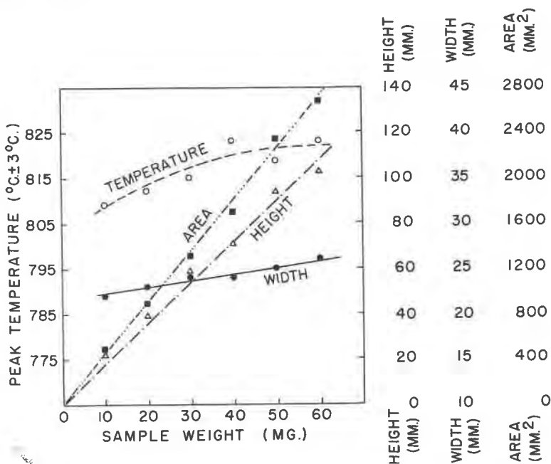
FIG. 4. Sample weight vs. peak dimensions. Peak height, width and area appear to be related linearly to the sample weight. Peak temperature decreases slightly below 40 mg.
