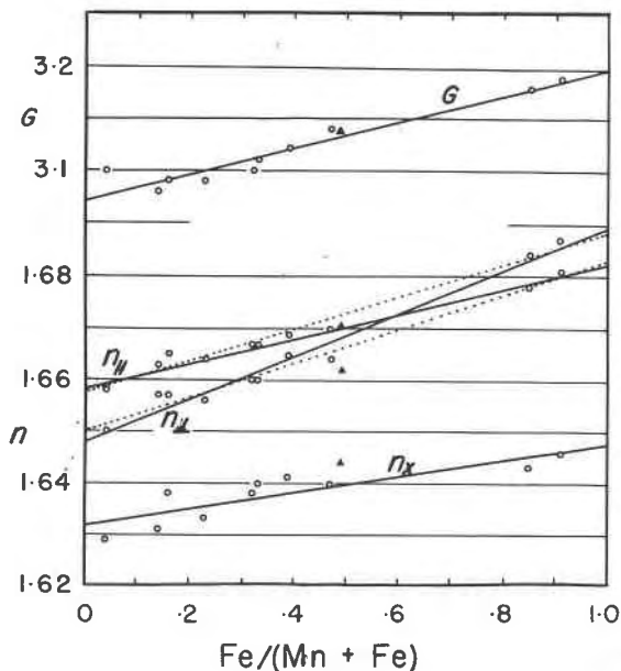
FIG. 1. Variations in physical properties in the Eosphorite—Childrenite series (modified from Hurlbut, 1950). The lines represent the regression equations (2) given in the text.
