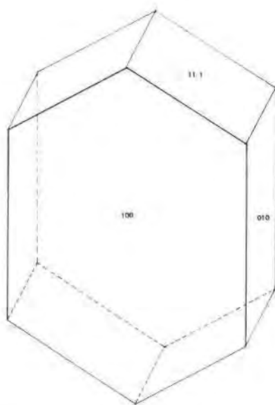
FIG. 2. Typical crystal of roscherite from the Sapucaia pegmatite mine.
