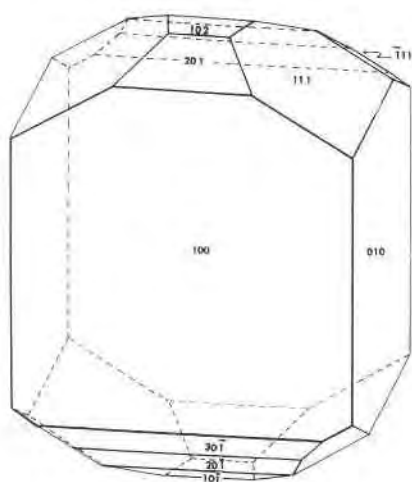
FIG. 3. Crystal of roscherite from the Sapucaia pegmatite mine showing development of the dome faces.
