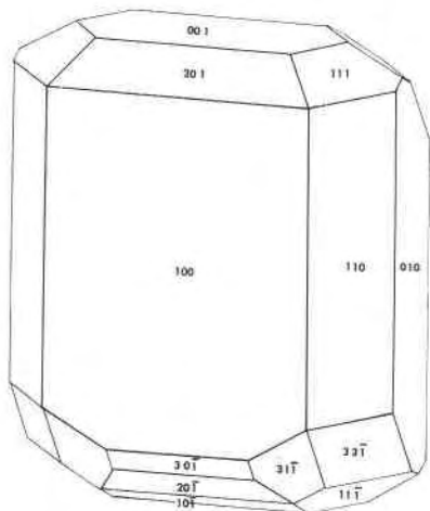
FIG. 4. Crystal of roscherite from Greifenstein, Saxony, showing full development of the terminating faces; typical crystals are usually segments of the prism zone.
