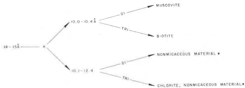
FIG. 2. Method of obtaining information pertaining to the origin of expanded minerals.
