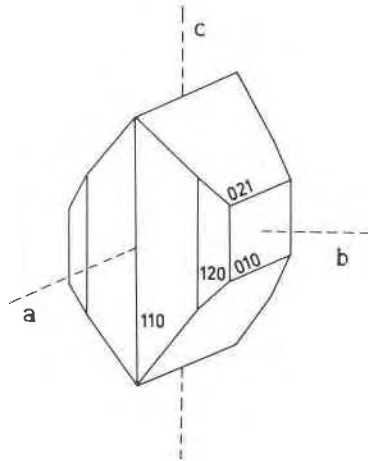
FIG. 2. The shape of the sub-calcium olivine crystals from Mt. Nyiragongo. Specimen R.G. 22778.
