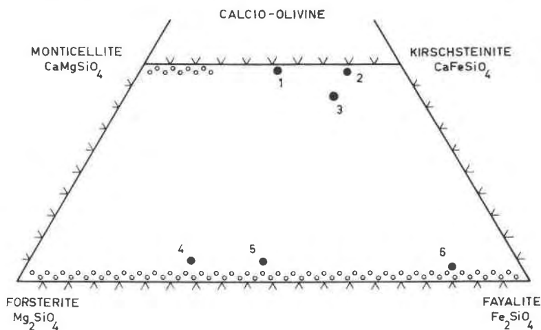
FIG. 1. The calcian-magnesian-ferroan olivines.
