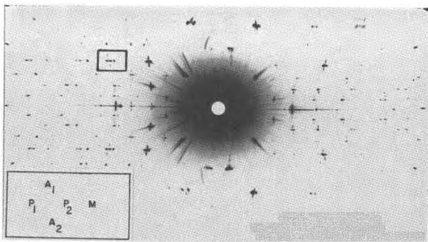
FIG. 5. Sanidine cryptoperthite from Cebolla, Creek, b axis oscillation photograph with the x -ray beam parallel to (001) in the center of a 15^\circ oscillation. The inset diagram in the bottom left hand corner provides a key for the interpretation of the reflections enclosed in the small rectangle in the upper left. There are five components: A_1A_2 and P_1P_2 are albite and pericline twins of the soda-rich phase and M is the monoclinic potash phase. The components are related by the M type of association because reflections P_1 and P_2 lie on the same layer lines whereas reflections from A_1 and A_2 lie on bent layer lines symmetrically related to the P_1P_2 layer lines. The b twin axis, therefore, is perpendicular to the (010) twin plane. The M reflections lie on the same layer lines as the P_1P_2 reflections indicating unmixing from an original homogeneous monoclinic phase.
