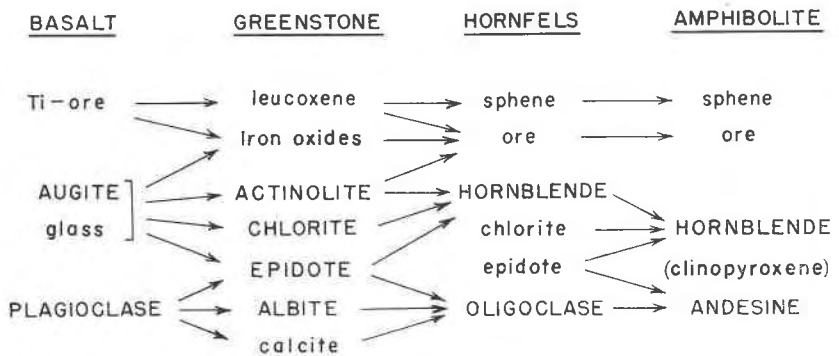
FIG. 1. Sequence of mineral assemblages in metabasaltic rocks of the Bidwell Bar region. The principal minerals are in capital letters.
