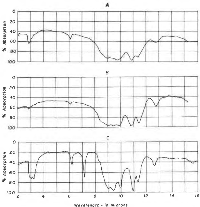
FIG. 1. Infrared-absorption spectra of natural and synthetic gastunite. A. Gastunite—Mammoth prospect, Presidio County, Texas. B. Synthetic potassium gastunite. C. Synthetic ammonium gastunite.
