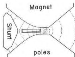
FIG. 3. Schematic transverse section through the magnetic field of a paramagnetic separator. The sample passes down the trough which is placed in the region of widest uniform divergence of flux line density.
