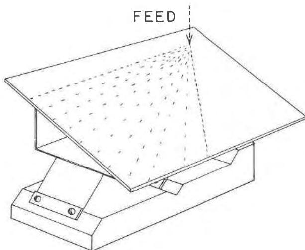
FIG. 5. The inclined-plane mica separator. The smooth aluminum table measures 11 \times 13 inches and slopes 15^\circ . It is mounted on the base of a commercial vibrating feeder.
