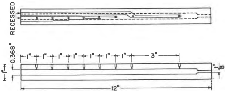
FIG. 4. Schematic diagram of stainless steel tube designed to fit in alumina tube of the temperature gradient furnace. Upper drawing is a plan view showing thermocouple wells and longitudinal grooves in which thermocouple leads were placed. Lower drawing is a cross-sectional view showing placement and shape of thermocouple wells.
