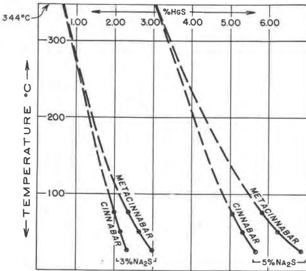
FIG. 2. The solubility of cinnabar (red HgS) and metacinnabar (black HgS) in 3% and 5% sodium sulfide solutions at 25° C., 50° C., and 75° C. as determined by Dickson and Tunell. Solid lines connect experimentally determined points, and broken lines represent curves extrapolated to intersect at the inversion temperature, 344° C.
