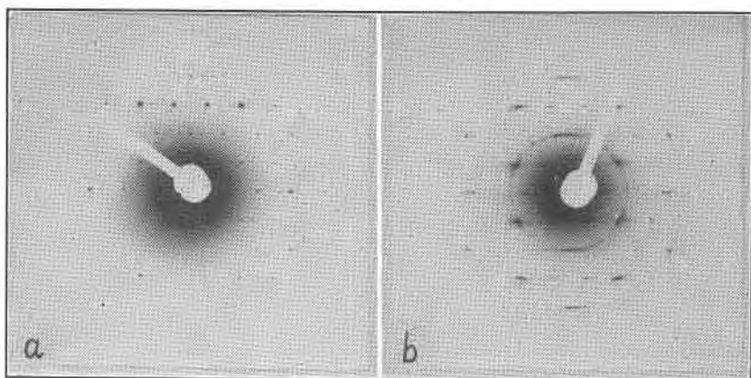
FIG. 2. Single crystal electron diffraction patterns of sepiolite from (a) Little Cottonwood, Utah, (b) Eski Chehir, Asia Minor.
