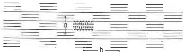
FIG. 3. Schematic representation of the cross-section of a sepiolite fiber, showing greater development in the b than in the a direction. The content of one unit cell is indicated schematically; the horizontal lines represent layers of oxygen atoms.
