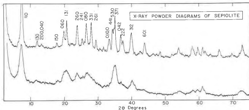
FIG. 1. X-ray diffractometer records of sepiolites from Little Cottonwood, Utah (upper curve), and Eski Chehir, Asia Minor (lower curve).
