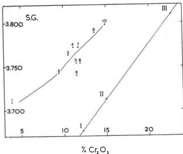
FIG. 3. Variation of specific gravity with chromium content. Bushveld uvarovite specimens—Arabic numerals. von Knorring's specimens—Roman numerals.
