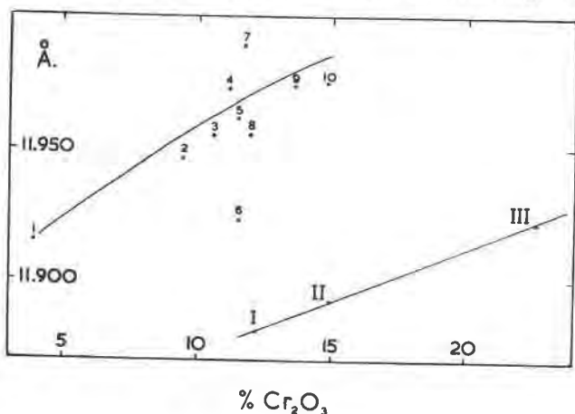
FIG. 2. Variation of unit cell with chromium content. Bushveld uvarovite specimens—Arabic numerals. von Knorring's specimens—Roman numerals.
