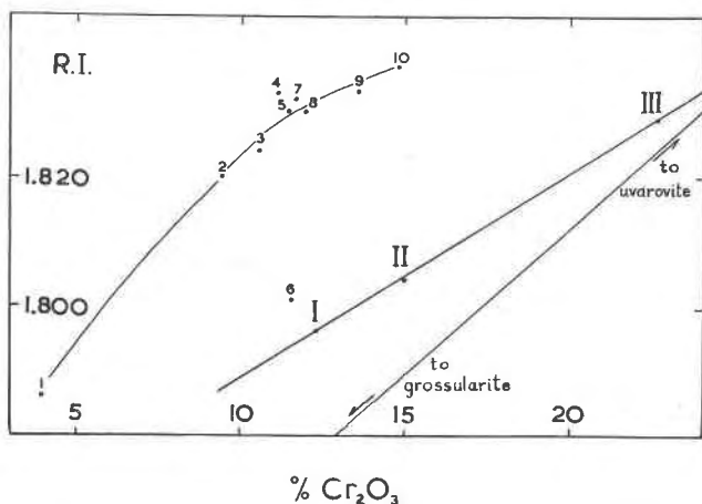
FIG. 4. Variation of refractive index with chromium content. Bushveld uvarovite specimens—Arabic numerals. von Knorring's specimens—Roman numerals.
