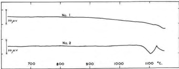
FIG. 5. Differential thermal analysis curves of (1) Uvarovite, de Kafferskraal, No. 359. (Table I, Analysis No. 7). (2) South African Jade, Buffelsfontein, No. 205. (Table VI, Analysis No. 1)
