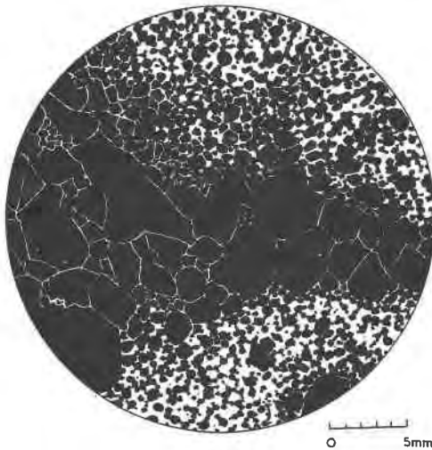
FIG. 7. Chain of large chromite grains in uvarovite-bearing chromitite. Locality Doornbosch, No. 423.
