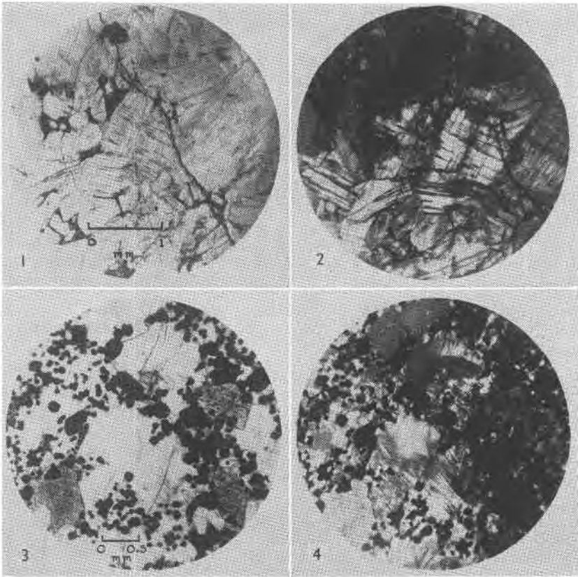
PLATE 2. (1) South African Jade in plane polarized light.
