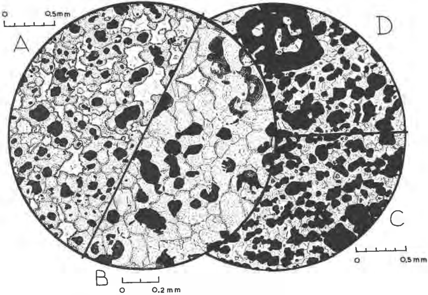
FIG. 6. A and B. Highly corroded chromite remnants (black) in uvarovite (stippled). Clear areas are mainly zoisite. Vygenhoek, No. 209. C. Chromite grains linked in short chains in uvarovite. A few small serpentinized olivine grains are present. de Kafferskraal, No. 359. D Corroded chromite grains in uvarovite. de Kafferskraal, No. 359.
