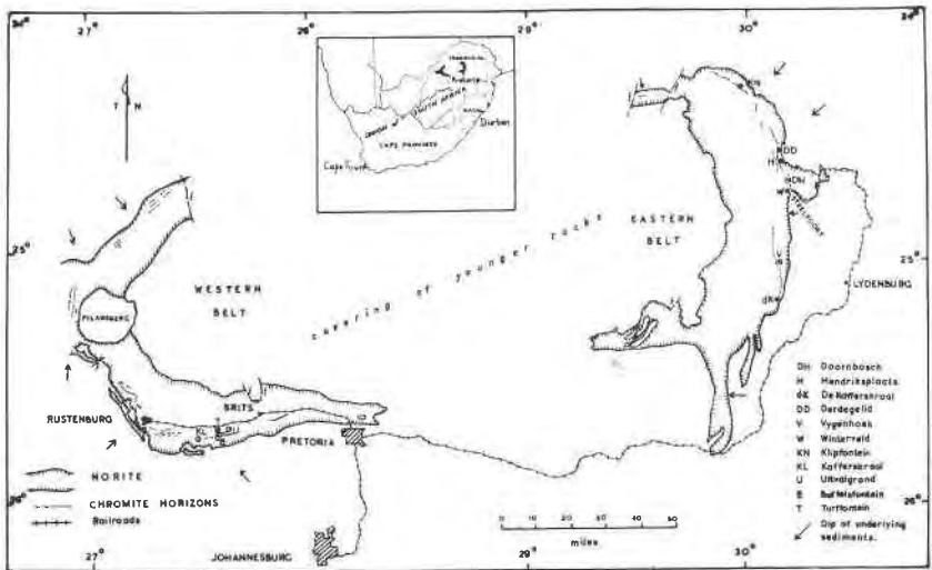
FIG. 1. Geological sketch map of the Central Transvaal, showing the extent of the Norite body of the Bushveld Complex and the localities of specimens here described. (Modified from Union Geological Survey Maps.)
