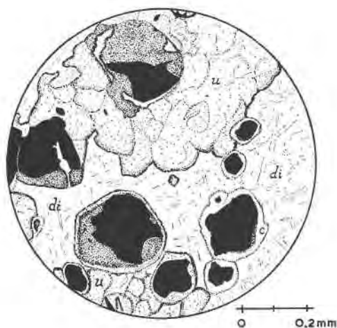
FIG. 8. Contact between diopside-rich band (di) and chromitite, showing corroded and replaced chromite (black) in green uvarovite (u), dark blue-green birefringent garnet (heavy stipple) and colorless chlorite (c).
