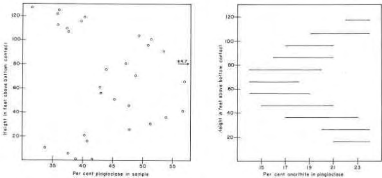
FIG. 7. Distribution of plagioclase in sill.
