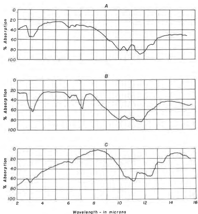
FIG. 2. Infra-red absorption spectra of natural and synthetic boltwoodite, and kasolite. A. Boltwoodite, La Chiquita mine, Quebrada del Tigre, Cordoba Province, Argentina, B. synthetic ammonium boltwoodite, C. kasolite, Shinkolobwe, Belgian Congo.
