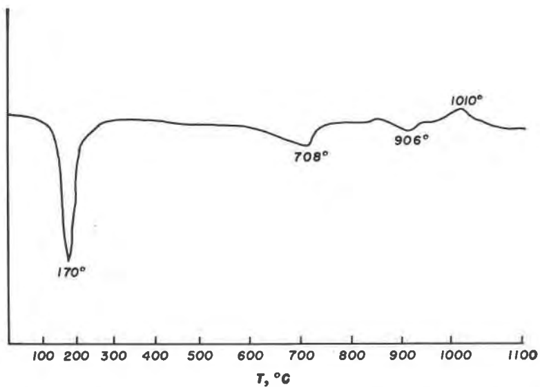
FIG. 3. Differential thermal analysis curve for boltwoodite from the La Chiquita mine, Quebrada del Tigre, Cordoba Province, Argentina.
